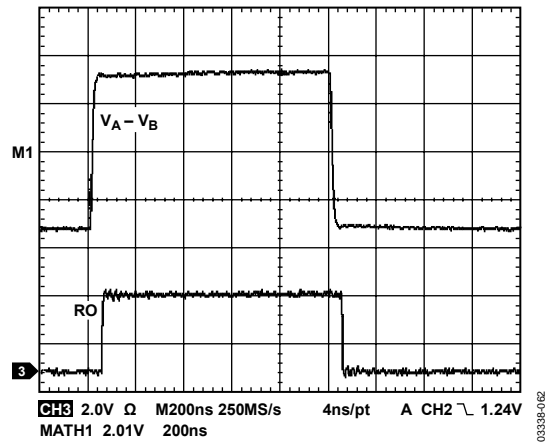
Figure 23. Receiver Propagation Delay, Driven by External RS-485 Device
