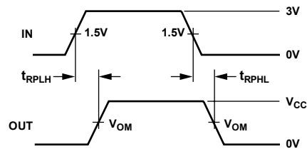
Figure 10. Receiver Propagation Delays
